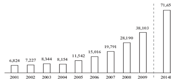
Newly installed global wind power capacity (MW)
